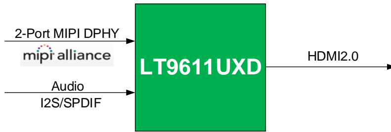
Figure 3.1 Application Diagram
