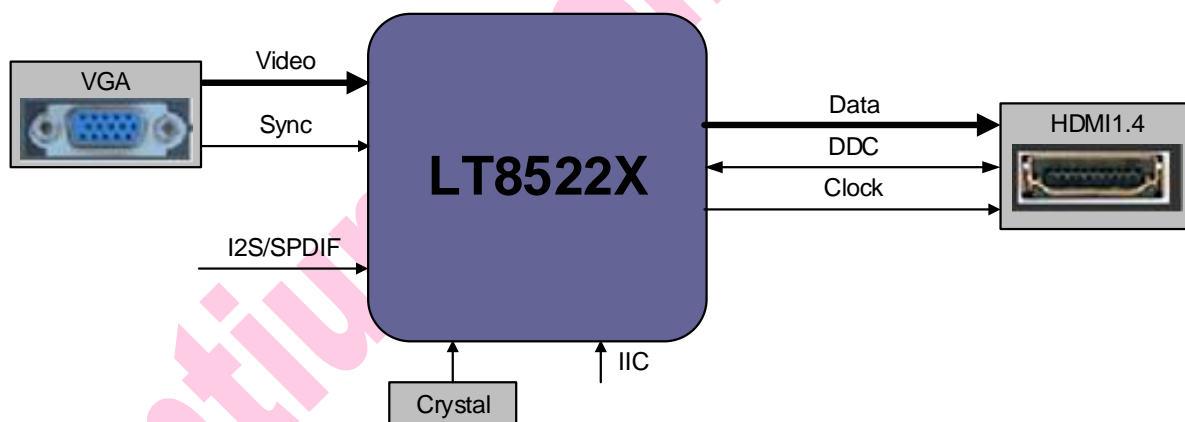
Figure 3.1 Application Diagram
