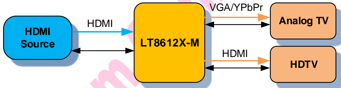
Figure 3.1 Application Diagram
