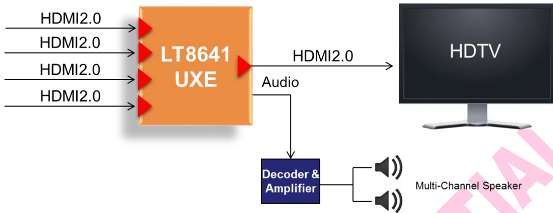
Figure 3.1 Application Diagram
