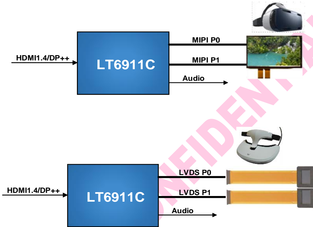
Figure3.1 Application Diagrams
