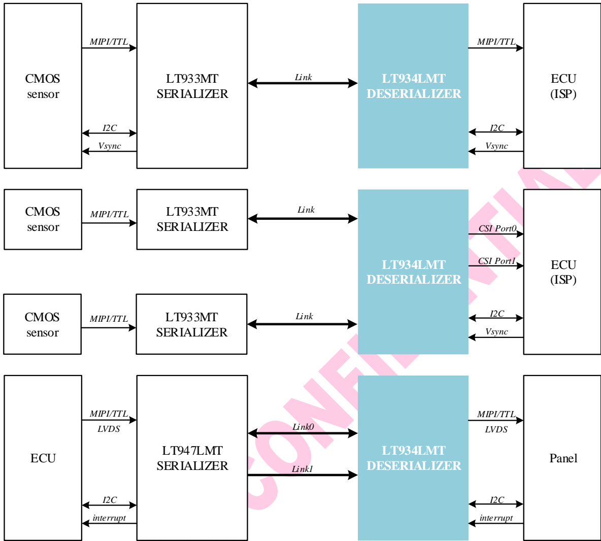
Figure 3.1 Application Diagrams
