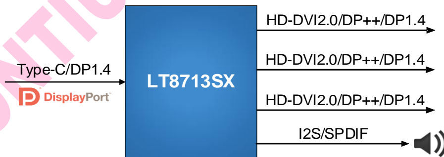
Figure 3.1. Application Diagram
