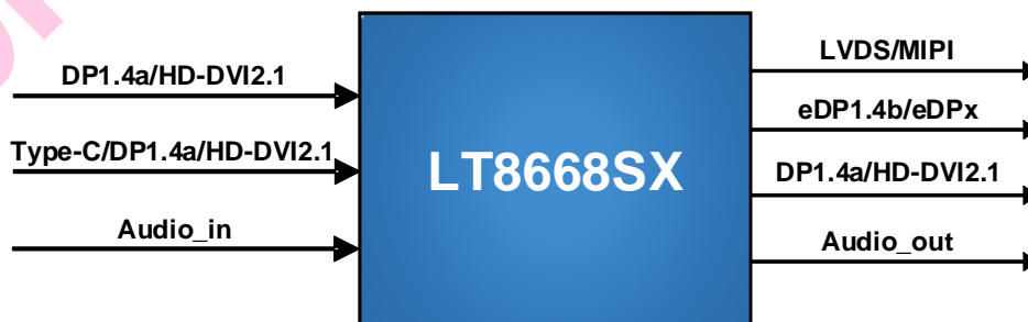
Figure 3.1 Application Diagram
